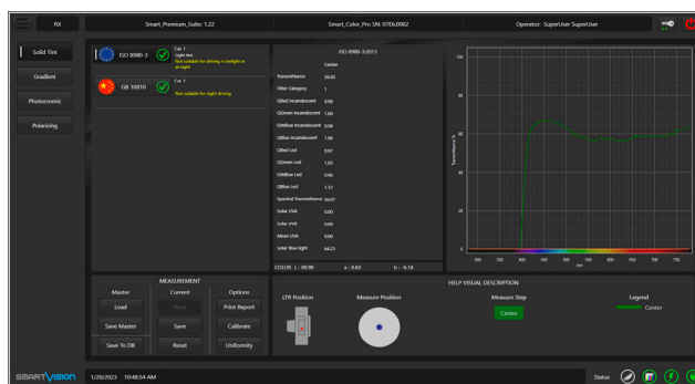
Ophthalmic (Optional) RX Plano Lens Conformity Check
